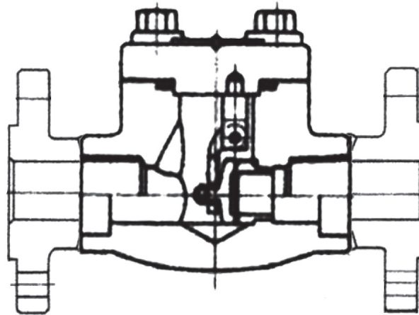
Flanged End Swing Check Valve
